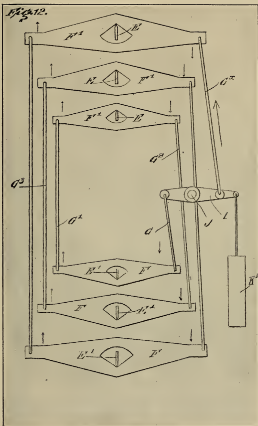
BANGERTER'S PERPETUAL TIME CLOCK
