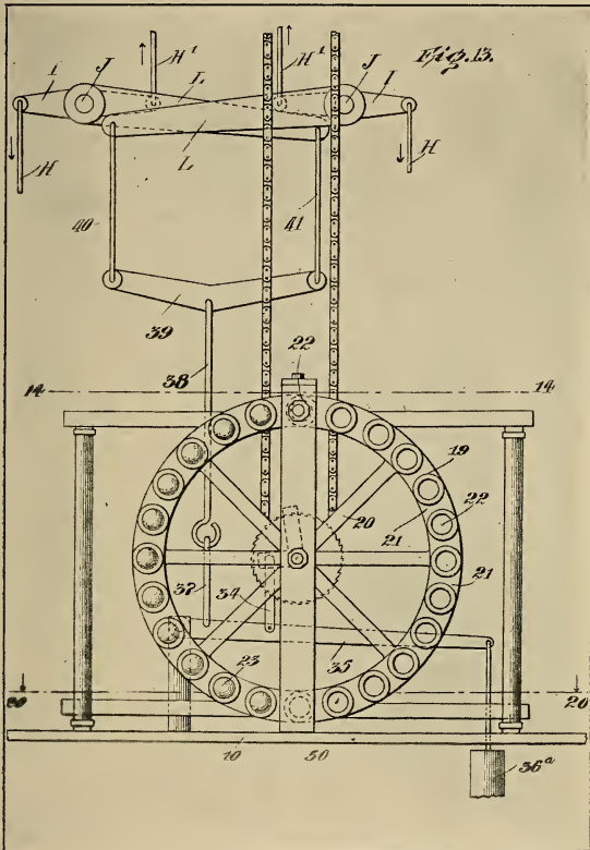
BANGERTER'S PERPETUAL TIME CLOCK
