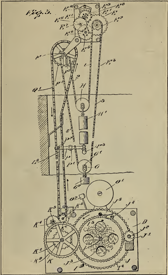
DRAWING OF BANGERTER'S SELF-WINDING CLOCK.
