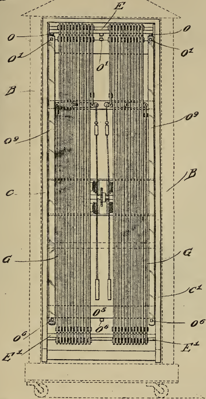
BANGERTER'S PERPETUAL TIME CLOCK
