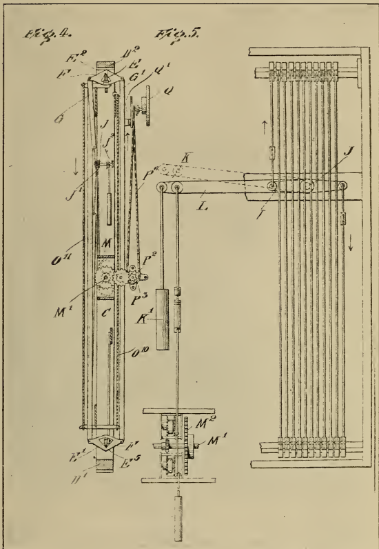
BANGTER'S PERPETUAL TIME CLOCK
