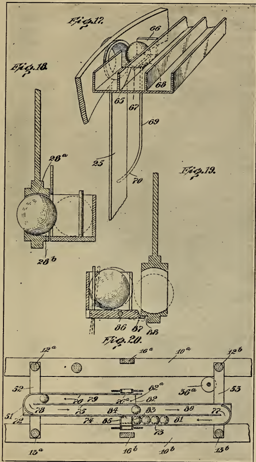
BANGERTER'S PERPETUAL TIME CLOCK
